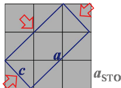
Figure 2. Planar view of the alignment of the \text{Sr}_4\text{Fe}_6\text{O}_{13} a - c plane of the film on to the \text{SrTiO}_3(001) plane of the substrate. The arrows indicate the expected compressive strain induced in the film by the substrate mismatch.
