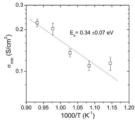
Figure 14. Dependence of the conductivity minimum \sigma_{\min} versus reciprocal temperature.
